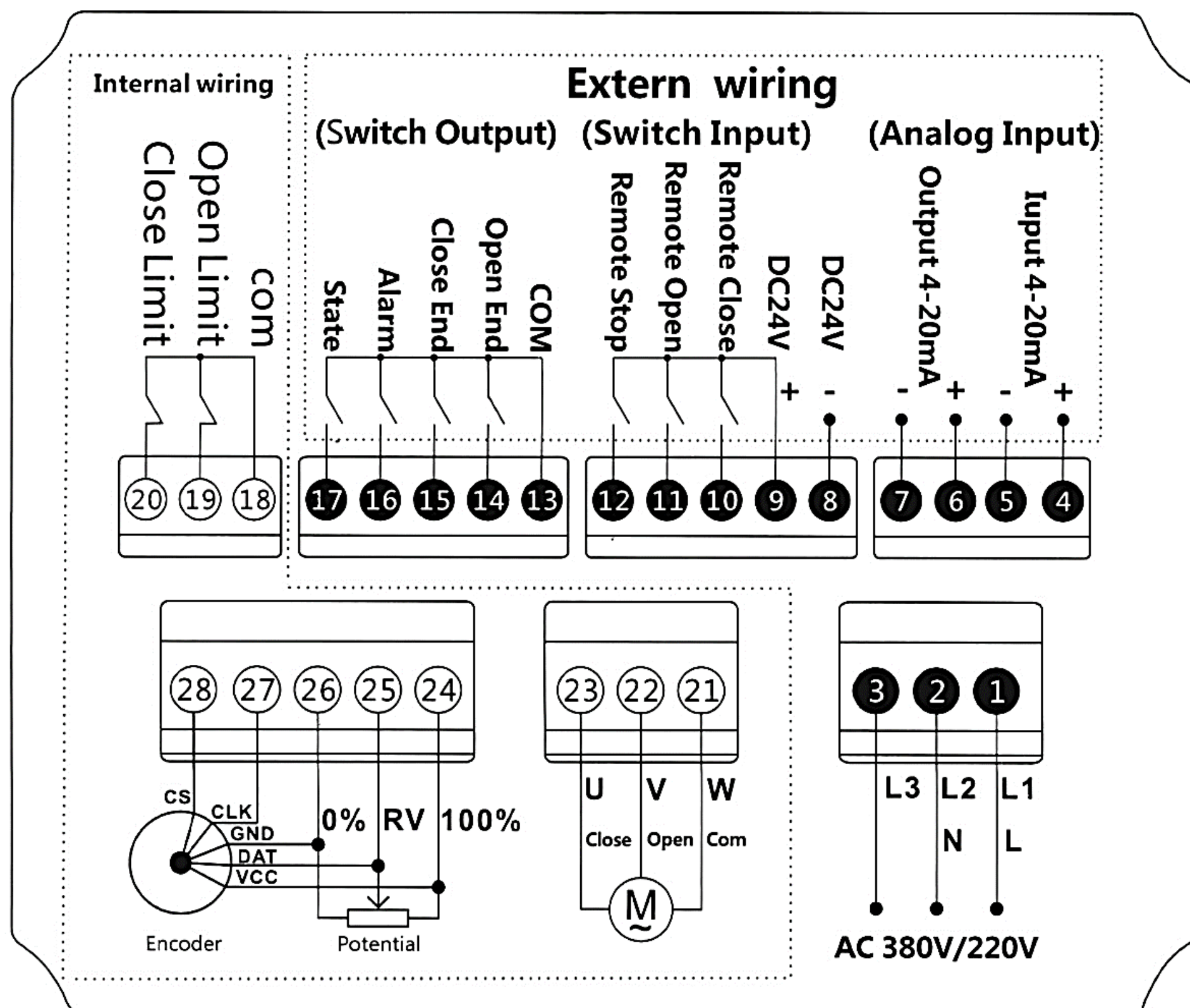
PICTURE 3 : SINGLE-PHASE / THREE-PHASE DIAGRAM
