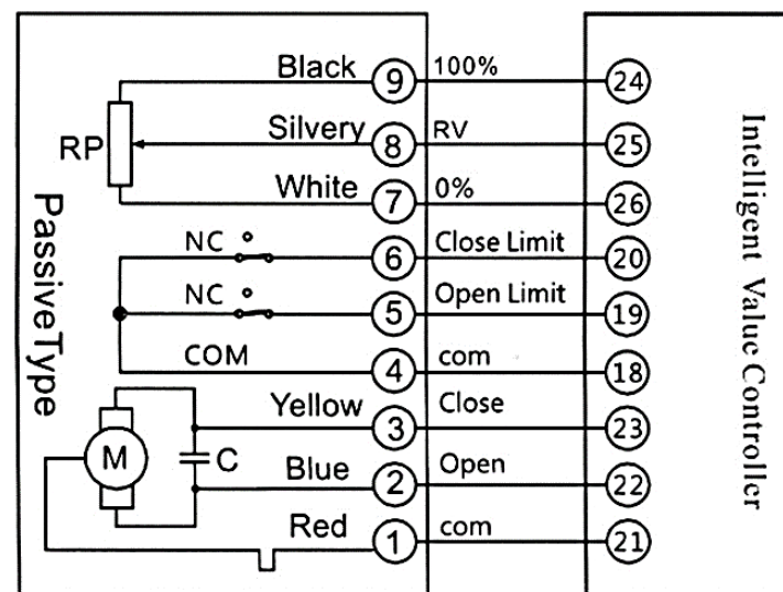
PICTURE 5 : WIRING OF THE PASSIVE CONTACT TYPE MOTOR (SETMD=2)
