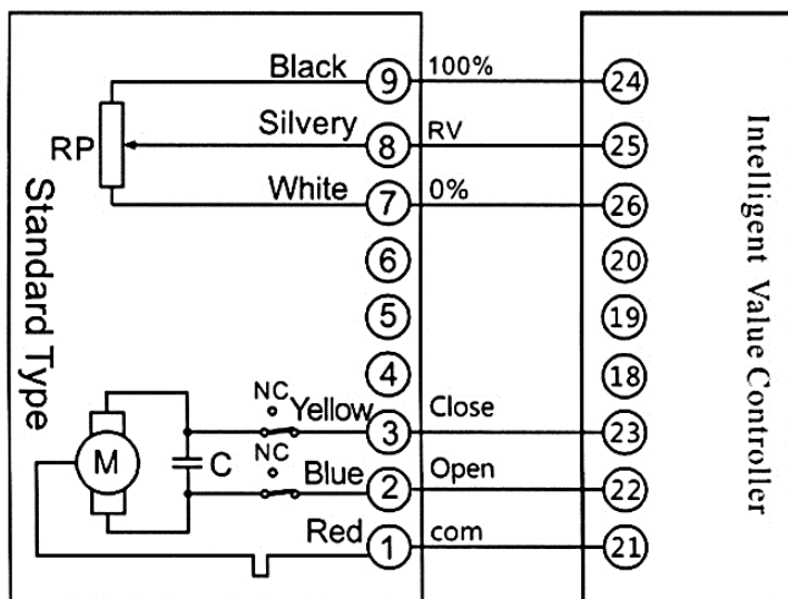
PICTURE 4 : WIRING OF THE STANDART ADJUST TYPE MOTOR (SETMD=1)
